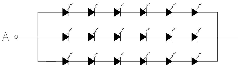
CIRCUIT DIAGRAM
